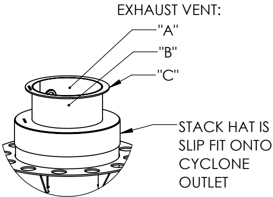
DETAIL D SCALE 1 : 8 EXHAUST VENT SEE TABLE 2
