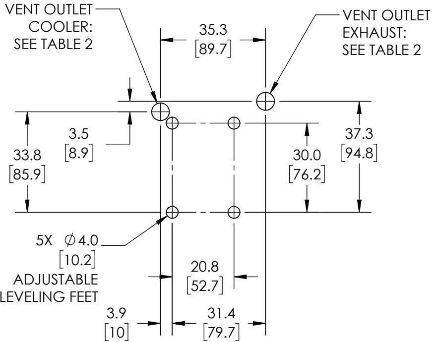
FOOT & VENT LOCATIONS TOP VIEW
