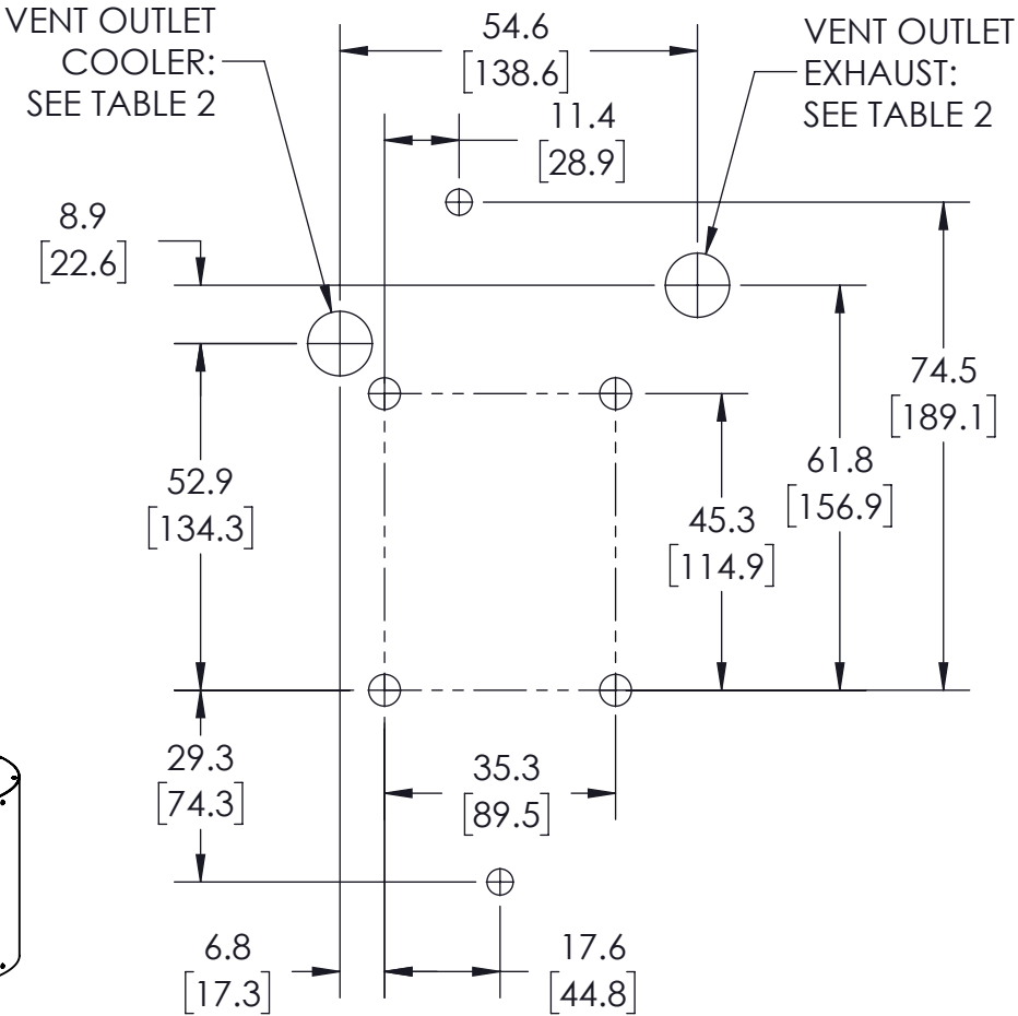
FOOT & VENT LOCATIONS
