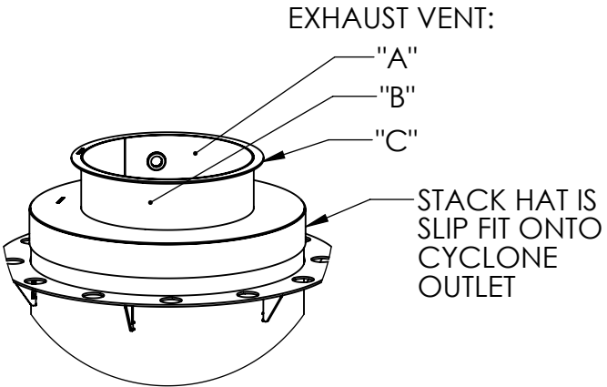
DETAIL C SCALE 1 : 10 EXHAUST VENT SEE TABLE 2
